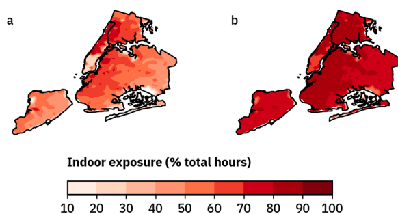
Fig. 5. Percent of summer (JJA) hours when indoor heat index reaches or exceeds Very Hot threshold in the (a) PRESENT and (b) FUTURE simulations.
